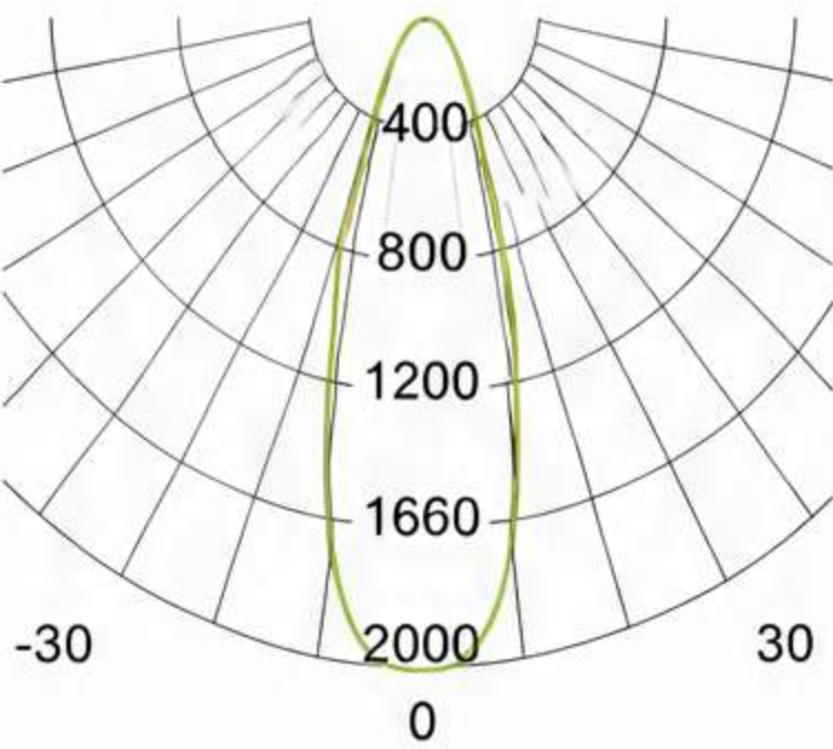
PHOTOMETRIC DIAGRAM
