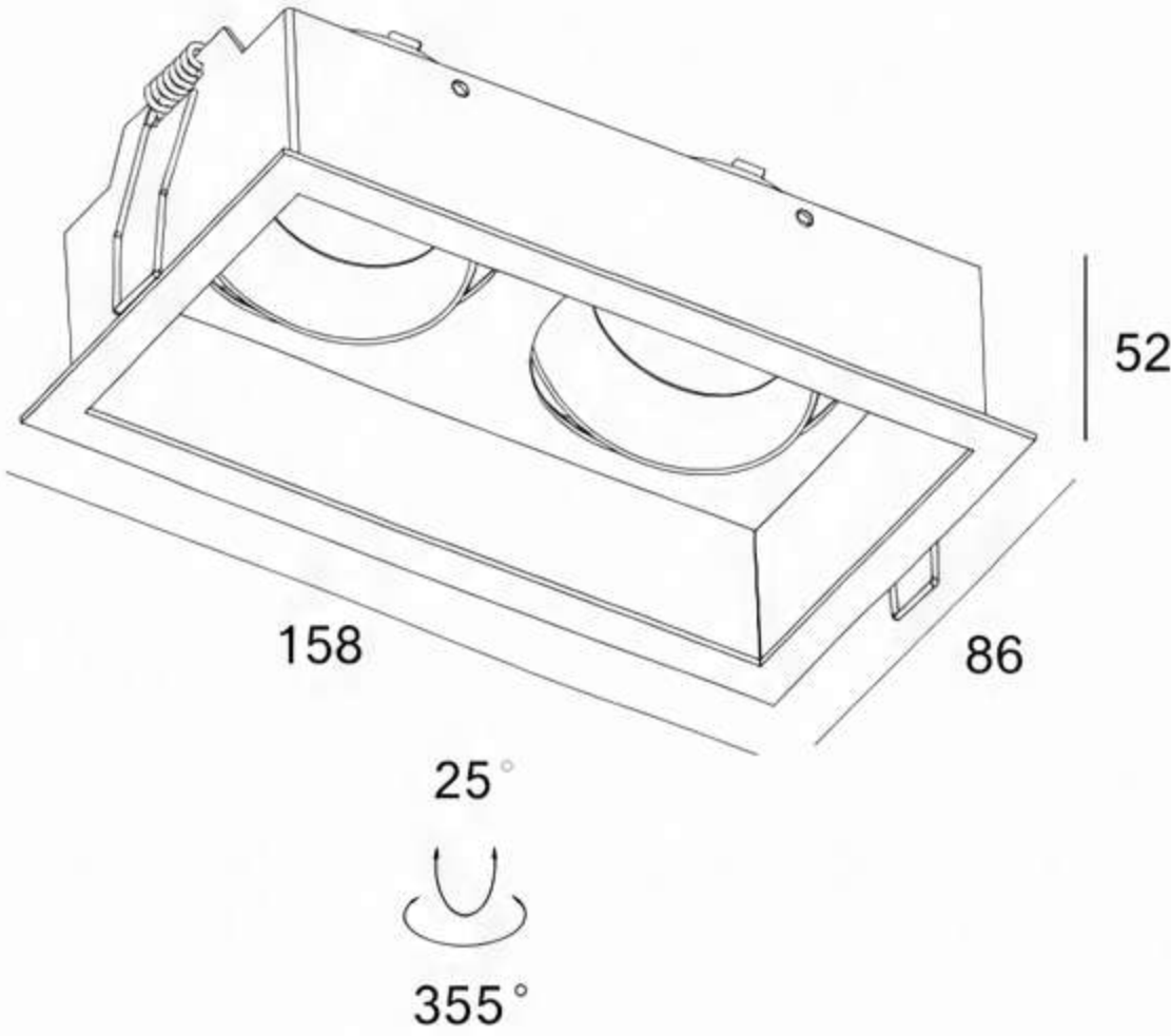
DIMENSIONS DRAWING
