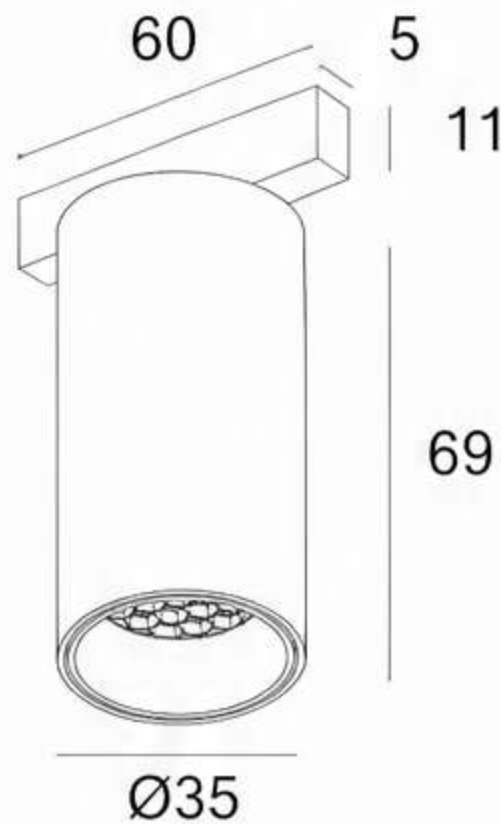
DIMENSIONS DRAWING
