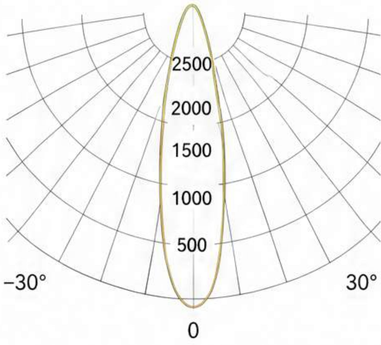
PHOTOMETRIC DIAGRAM
