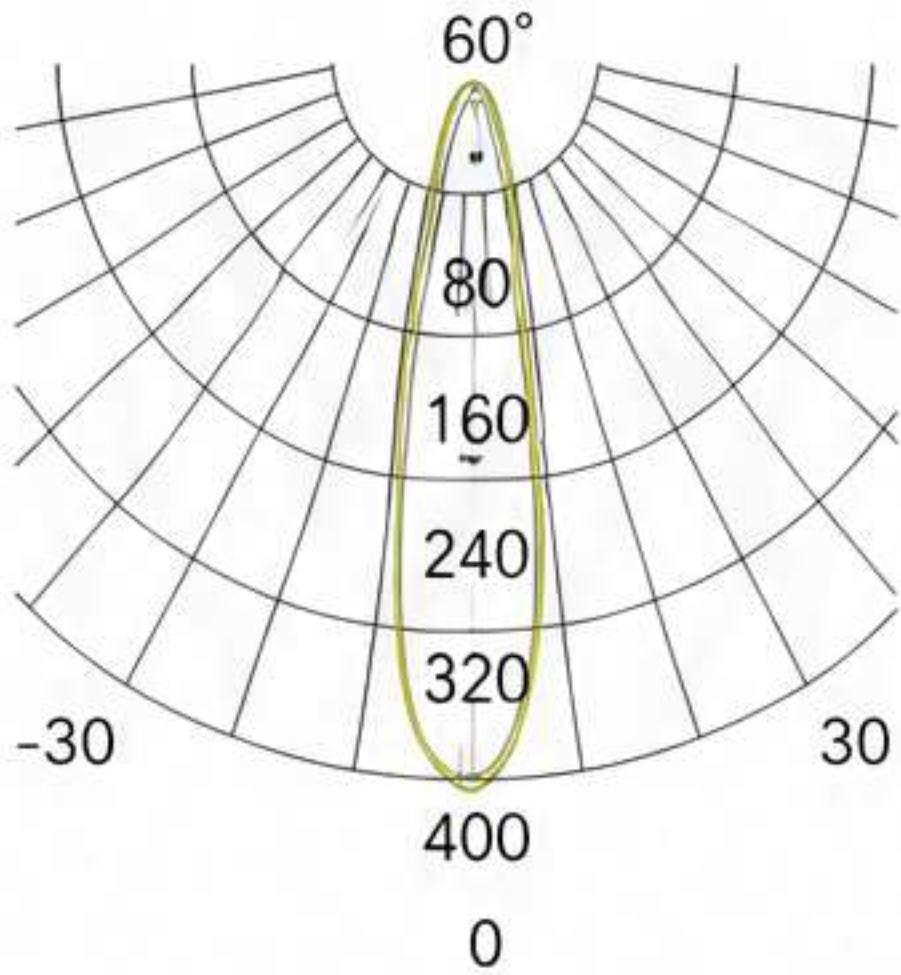
PHOTOMETRIC DIAGRAM
