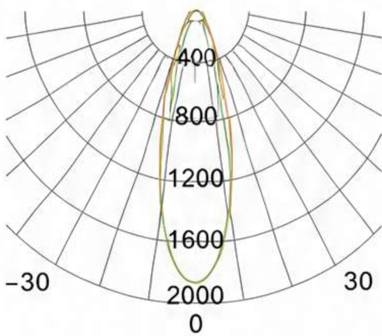
PHOTOMETRIC DIAGRAM
