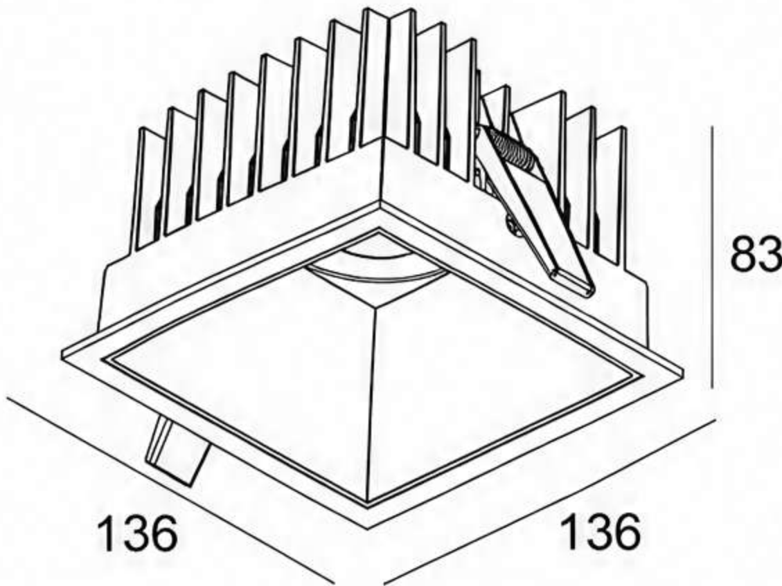
DIMENSIONS DRAWING
