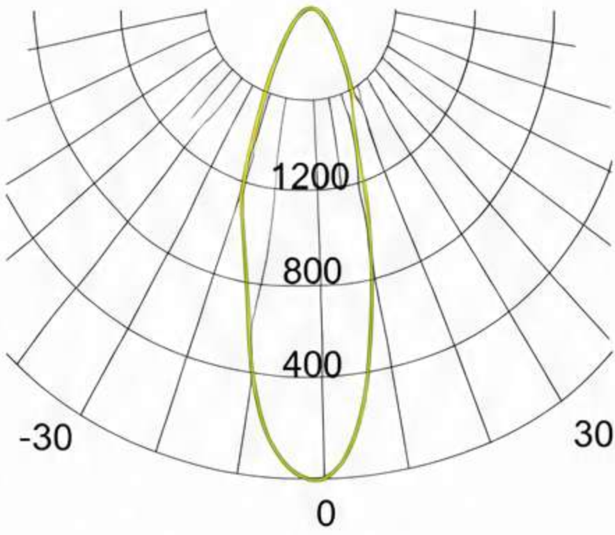
PHOTOMETRIC DIAGRAM
