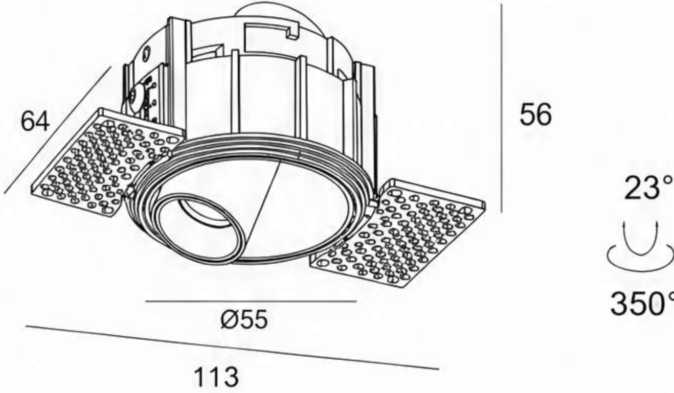
DIMENSIONS DRAWING
