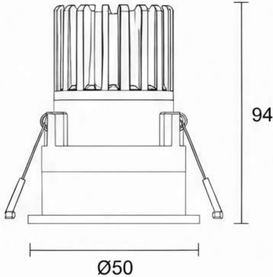
DIMENSIONS DRAWING
