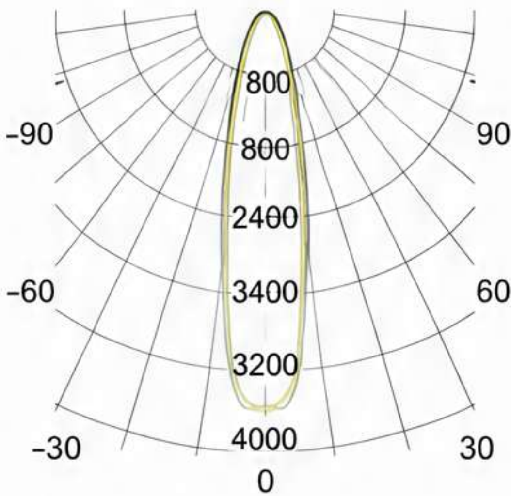
PHOTOMETRIC DIAGRAM
