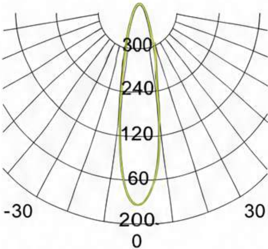
PHOTOMETRIC DIAGRAM
