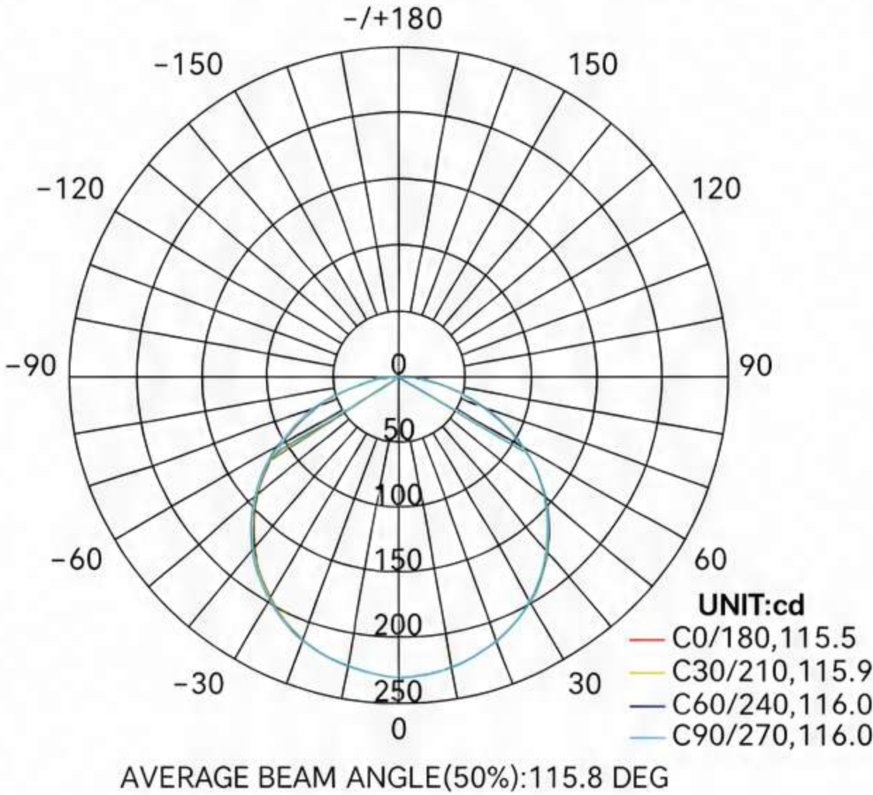
PHOTOMETRIC DIAGRAM
